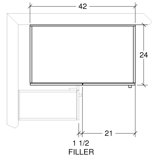
Hafele Magic Corner II cabinet size: 42" wide x 24" deep
