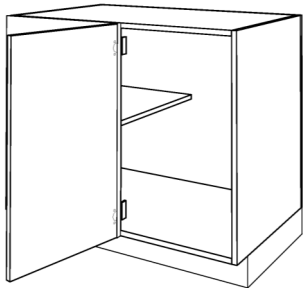
blind corner box door widths (A): 15" 18" 21" 24"
